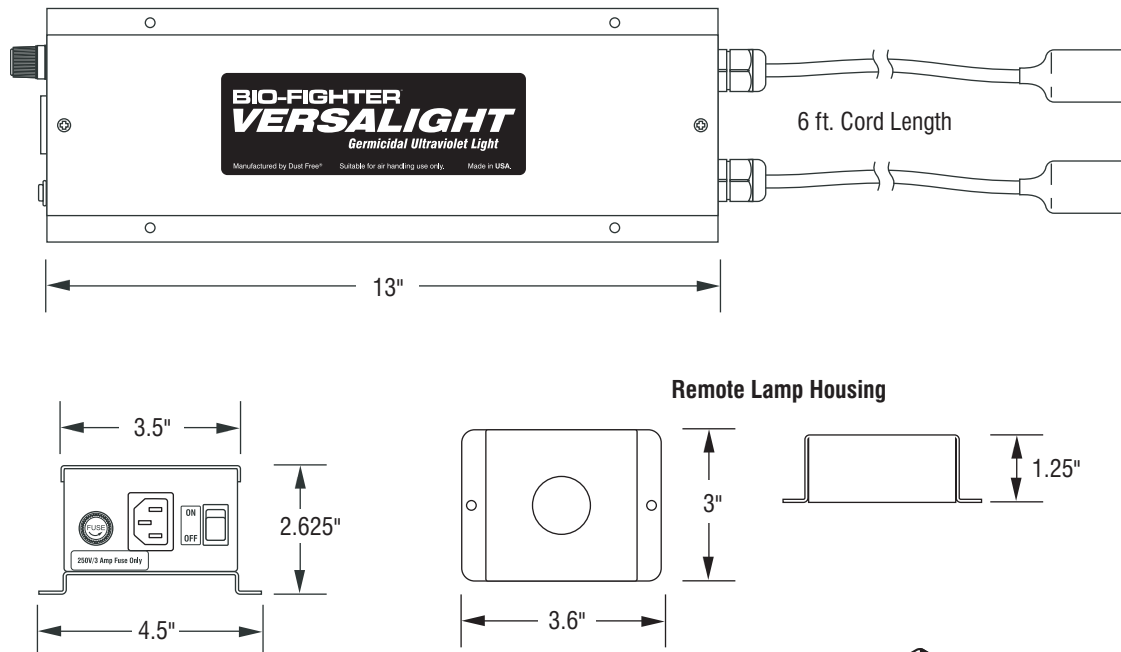
Fig. 1 Dimensions of single and dual lamp VersaLights.
